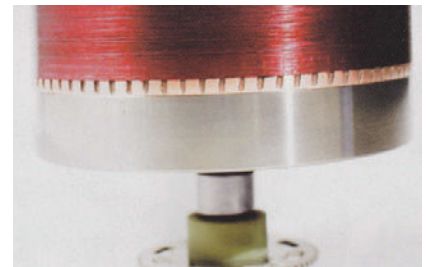
Copper Rotor Propulsion Motor in Tesla's Powertrain
