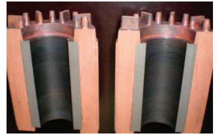
Cross-section Through Rotor Bars and End Ring of Die Cast Copper Rotor
